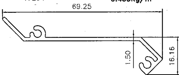
17254 0.435Kg/m
