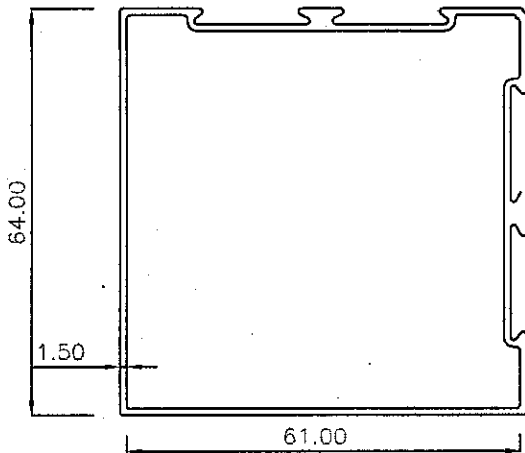
17254 0.435Kg/m
